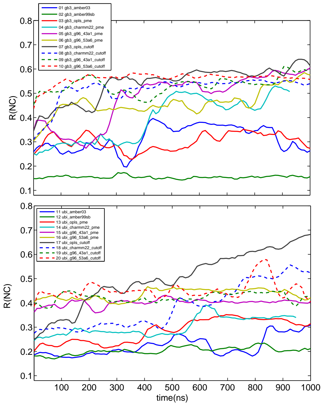
FIGURE S19. Time resolved NC - R_{RDC} for MD simulations with various force-fields. The residual dipolar couplings were computed from the respective MD trajectory in (overlapping) windows of 50 ns length.
