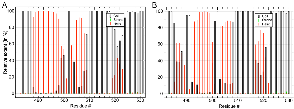
Figure 12: Secondary-structural stability in Molecular-Dynamics simulations as shown in Figure 4 of the Main Manuscript. A) SREBP-1 equilibrated in DLPC membranes. B) SREBP-1 equilibrated in membranes with exchange of the environment against water. Random coil, \beta -strand, and \alpha -helical structure are represented as black, green, and open red bars, respectively. The relative extent of the different types of secondary structure over time were extracted from Amber calculations over 760 and 900 ns in A) and B), respectively, with equidistant snapshots spaced by 0.4 ns.
