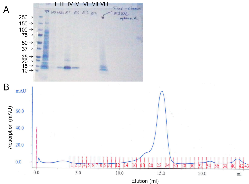
Figure 2: Typical outcome of SREBP purification. A) Metal affinity chromatography of the refolded cell-free SREBP full-length anchor precipitate. Lines I to VII represent throughflow, wash fractions with 0 and 20 mM imidazole, and 4 elution fractions of 1 CV each on gravity-column Nickel resin. Fraction VIII shows an (incomplete) Thrombin cleavage at room temperature. In later stages of the project, Talon resin was used rather than Nickel beads due to better compatibility with reducing agents. B) Monodisperse profile of the anchor in size exclusion chromatography on an analytical S200 column. The use of SEC was observed to provide hardly any sample improvement and was usually omitted in later stages of the project.
