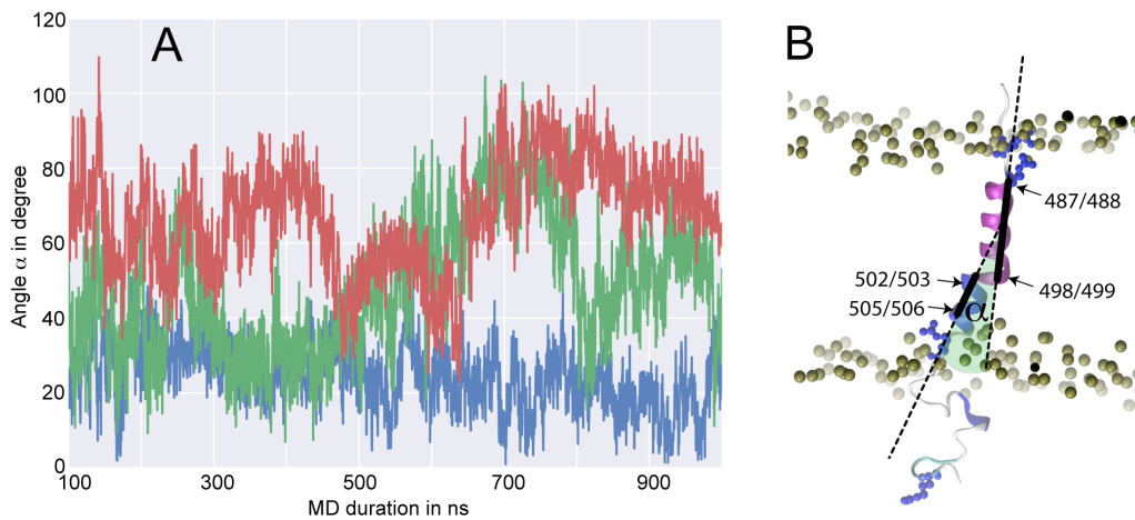
Figure 13: Fluctuations of the hinge-motional angle of the SREBP anchor in MD simulations using an Amber99sb-ILDN force field. The green, blue, and red curves signify the angle measured between the first and second helical part above and below the hinge motif in DLPC, POPC, and water environment, respectively. The hinge angle is defined here as the angle between two vectors in the helix direction, i. e. i) the vector connecting the mean between C^\alpha of residues 487 and 488 with the mean between C^\alpha of 498 and 499 and ii) the vector connecting the mean between C^\alpha of residues 502 and 503 with the mean between C^\alpha of residues 506 and 507.
