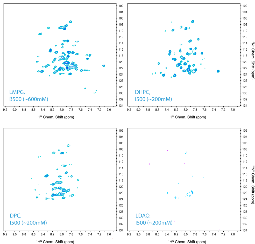
Figure 3: Detergent screens at 500 MHz proton Larmor frequency. Shown are spectra of the full-length SREBP anchor expressed without a histidine tag recorded in lyso myristoyl glycerophosphoglycerol (LMPG), dihexanoyl-glycerophosphocholin (DHPC), dodecyl phosphocholin, and lauryldimethylamine oxide (LDAO) in 7 h each. The spectrum in LMPG was recorded using a 600 mM sample and a room temperature probe, whereas the others were recorded on 200 mM samples using a spectrometer equipped with a cryoprobe.
