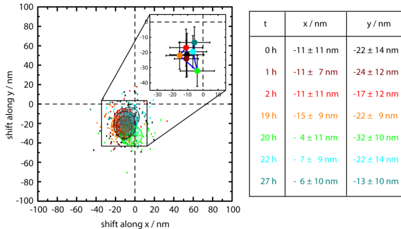
Fig. 6. . Stability of the dual-wavelength colocalization measurements. The main scatter plot shows the offset of individual beads between the two color channels at various times. The inset shows the image offset as obtained by averaging over the individual offsets. Over the whole measurement period the offset remains constant to within the statistical error of the experiment.
