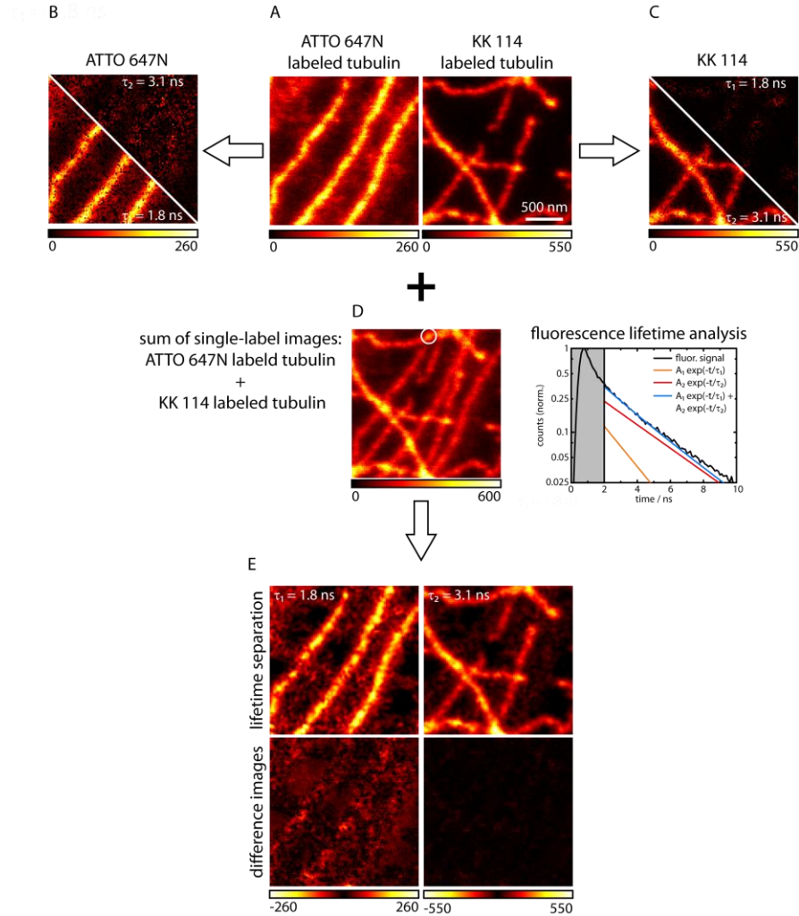
Fig. 2. Fluorescence separation by lifetime analysis. Images of tubulin labeled with ATTO 647N (left) or KK 114 (right) were recorded by TCPSC (A). A per-pixel monoexponential fit of the lifetime histogram reproduces the original images with residuals < 10% (B, C). Even after adding the photocounts of the original recordings (D) the two channels can be recovered by fitting a biexponential function to the lifetime histograms: (E) shows the amplitude images (top) of the two lifetime components along with the corresponding difference to the initial data (bottom).
