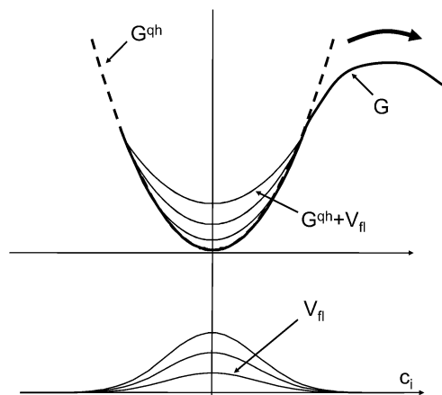
FIGURE 1 Action of the flooding potential. The lower part shows the flooding potential V_{\text{fl}} , with different curves corresponding to different values of the flooding strength E_{\text{fl}} . The upper part shows the free energy landscape G along a generalized coordinate c_i (bold line), its local quasiharmonic approximation G^{\text{qh}} (bold dashes) and the flooded landscape once the potential has been applied (thin lines, different E_{\text{fl}} values). Inclusion of the flooding potential within the force field effectively lowers free energy barriers and accelerates conformational transitions.
