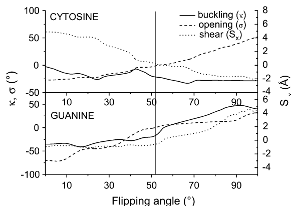
FIGURE 12 Variation of the buckling, opening ( ^\circ ) and shear ( \text{\AA} ) parameters as a function of the flipping angle. The thick vertical line materializes the average closed-state conformation.
