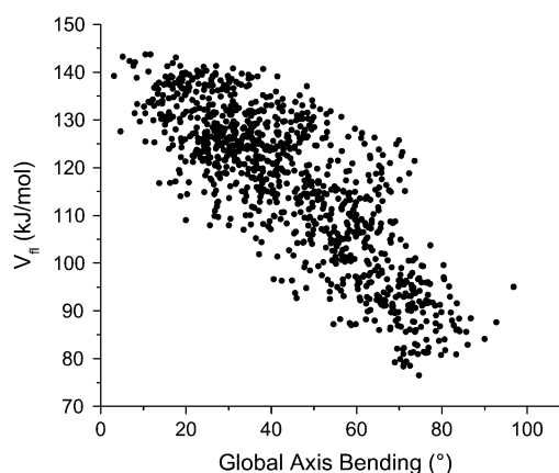
FIGURE 4 A flooding potential built upon the first five PCA eigenvectors, with E_n = 35 kcal/mol, induces exaggerated bending of the DNA helix. Each point represents a snapshot from a flooding simulation and is associated with a global helical bend angle and a flooding potential value; these two parameters can be seen to exhibit opposite variations.
