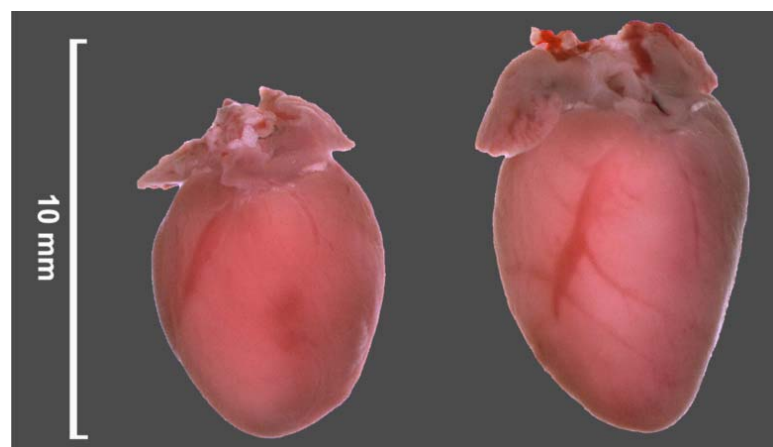
The hearts of the mice that possess more of the microRNAs 212 and 132 (on the right) are distinctly larger than the hearts of the normal mice (on the left). (Image: Kamal Chowdhury / Max Planck Institute for Biophysical Chemistry)
