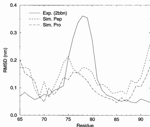
Fig. 6. RMSD of the C_{\alpha} atoms of the CaM central helix which were averaged per residue over the first 500 ps of the Sim. Pep and the entire Sim. Pro simulations. Also shown is the RMSD for C_{\alpha} atoms from NMR structure of CaM complexed with peptide from MLCK (Ikura et al., 1992).
